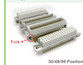
DG1120-01 Series DIN 41612 R Type 3 Row V/T & R/A Type W/ Fork
