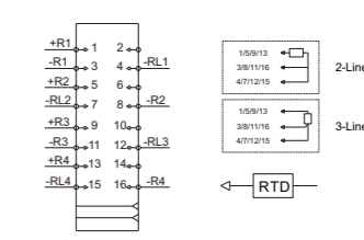
DF20-M-4RTD-PT
