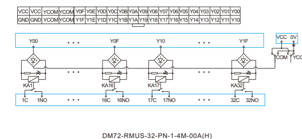
DM72-RMUS-32-PN-1-4M-00A(H)
