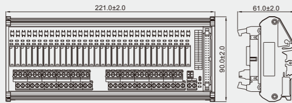
DM72-RMUS-32-PN-1-4M-00A(H)
