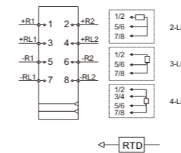
DF20-M-2RTD-PT
