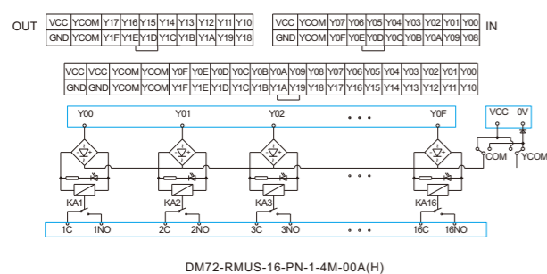
DM72-RMUS-16-PN-1-4M-00A(H)
