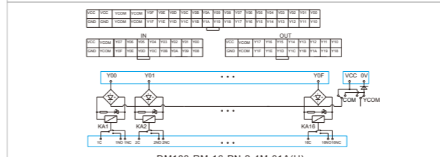
DM108-RM-16-PN-2-4M-01A(H)
